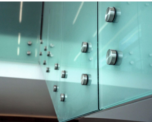
Stainless steel "buttons" pass through the glass and are bolted into the fascia for a clean, minimalist look.
