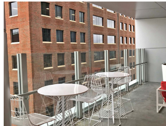
Ascent is post-supported and attached using baseplates with epoxy anchors, as seen on the north side of the building.
