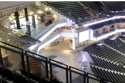
Upper fan seating area utilized painted aluminum railing with perforated infill.
