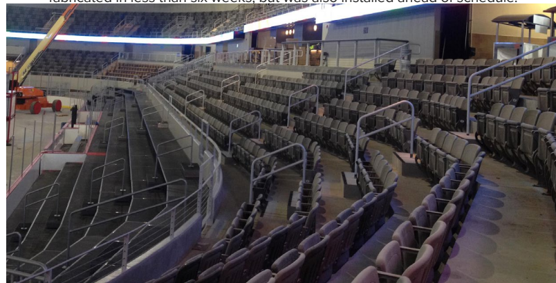
Sightline's product was designed to fit between a newly constructed dasher board system for the ice rink setup and concrete stadia that had existing fixed seating.
